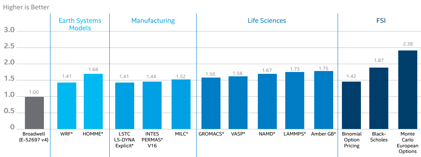
Across 13 common HPC workloads, Intel® Xeon® Scalable platform delivers improved performance.
